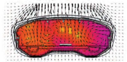
Figure 9.1. Original Venting Pattern
