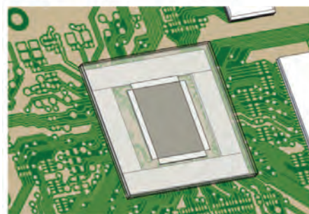
Figure 3. Component Level Modeling
