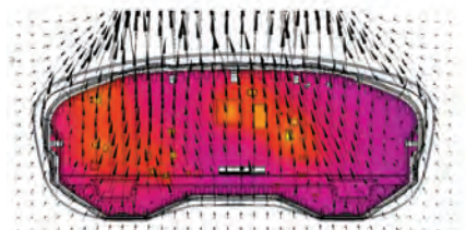
Figure 9.2. Wider Venting Pattern
