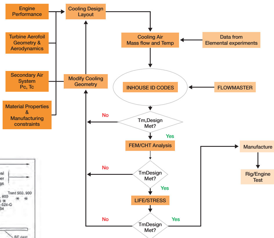
Figure 2. GTRE Design Loop
