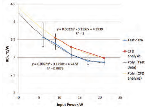
Figure 15. Performance of V8 in Vertical Up Orientation
