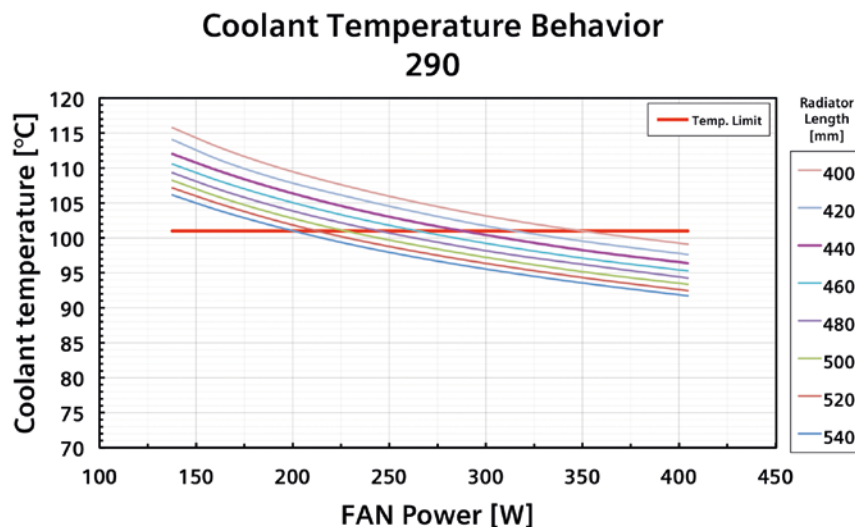
Figure 5: Coolant temperature, A test case
