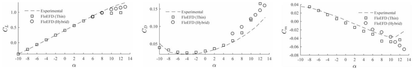
Figure 4: Comparison of Lift, Drag and Pitching Moment coefficients
