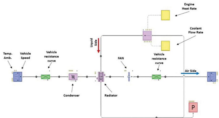
Figure 3: Simcenter Flomaster Cooling Model
