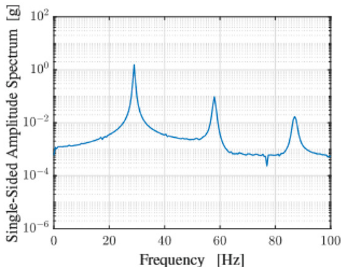
Figure 9: 0.1-g base level test, FFT over [163, 165] s of the notching channel
