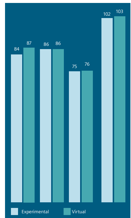
Figure 4: Model validation of temperatures
