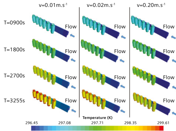
Figure 2: The temperature rise in the first set of series cells in the pack is a function of the 0.9 (°C) discharge rate and contact resistance of 0.0025 (m 2 ·°K)/W.
