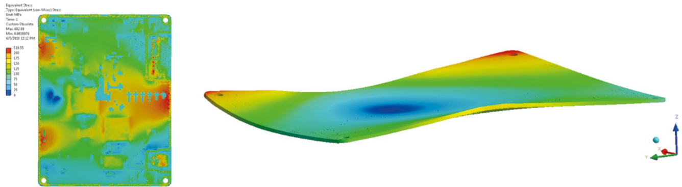
Figure 3: Von-Mises stress and out-of-plane deflection of detailed board with components modeled
