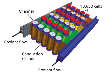
Figure 1: Geometry of the pack and the thermal management system.
