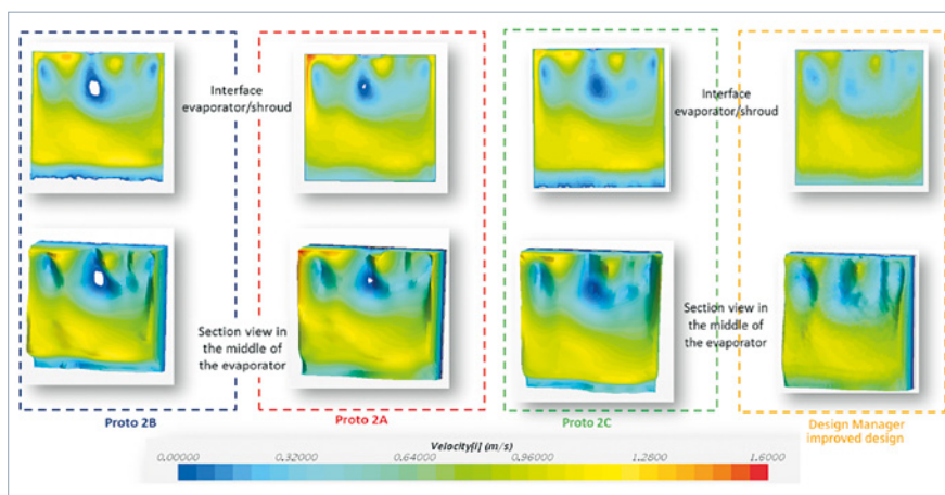
Figure 8: Comparison of velocity distribution at the evaporator interface.
