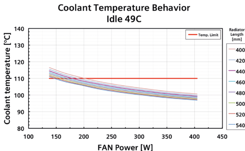
Figure 7: Coolant temperature drive scenario G test case
