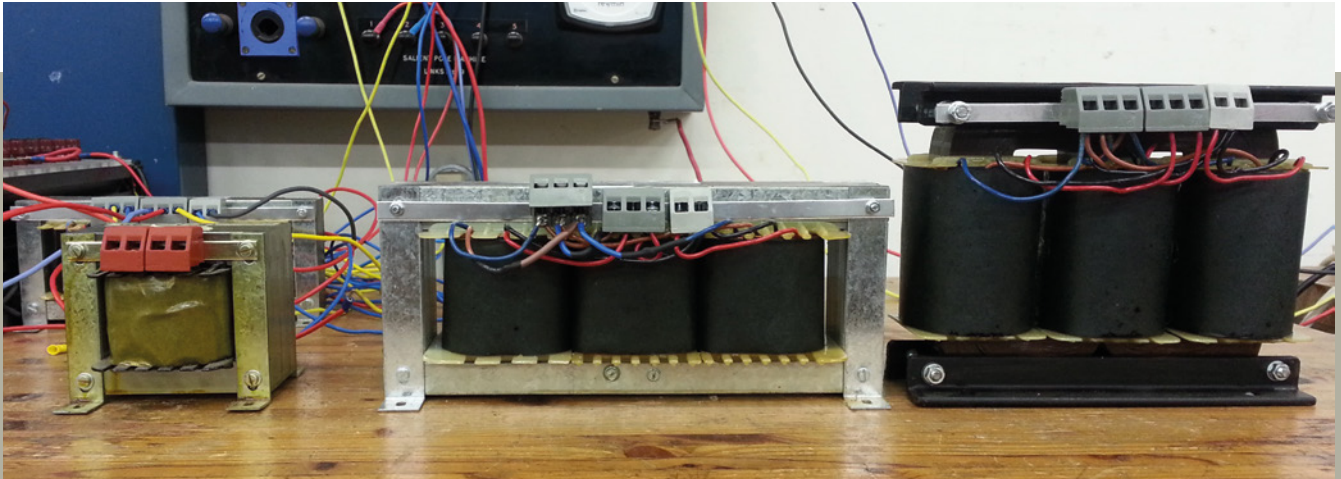
Figure 1. Bench-scale transformers single-phase shell type (left) three-phase five limb (centre) and three-phase three limb (right).
