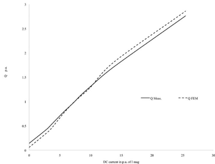
Figure 3. Measured and simulated reactive power Q in per unit (p.u.) of the VA rating vs. DC in p.u. of the transformer magnetizing current ( I_{mag} ) for 1p3L laboratory transformer.
