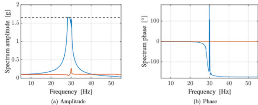
Figure 7: Spectrum verification for 0.1-g base level test using harmonic filtered with Simcenter Testlab
