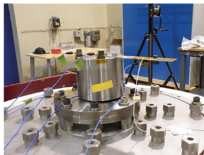
Figure 1: Test rig and numerical model for fixed / free beam
