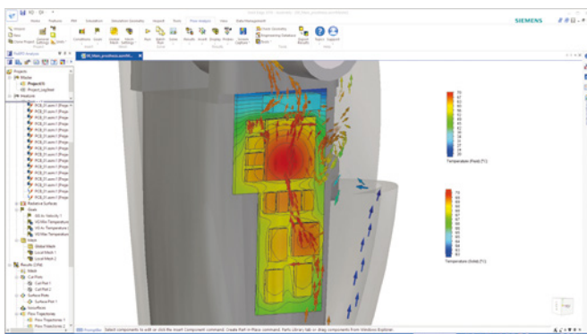
Figure 5: Temperature distribution on the PCB
