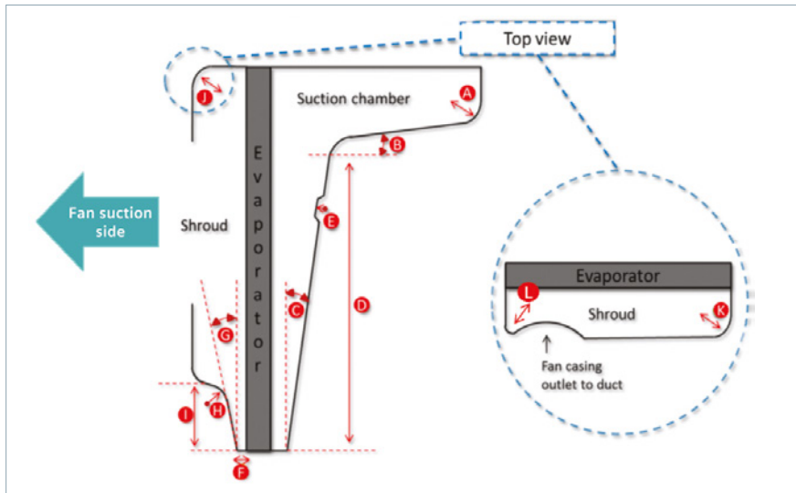
Figure 4: The 12 design parameters used in the Simcenter STAR-CCM+ Design Manager study.
