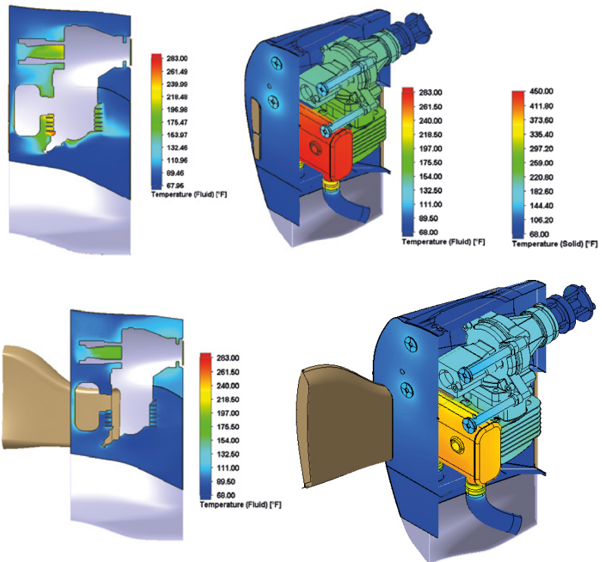
Figure 6: Comparison of temperature distribution (fluid and solid) for the engine assembly with and without ducts .
