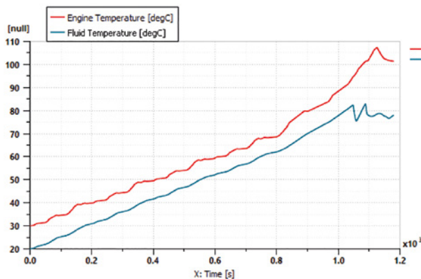
Figure 4: Simcenter Flomaster provides Simcenter Amesim with values of engine temperature, fluid temperature downstream of the engine and pump torque.
