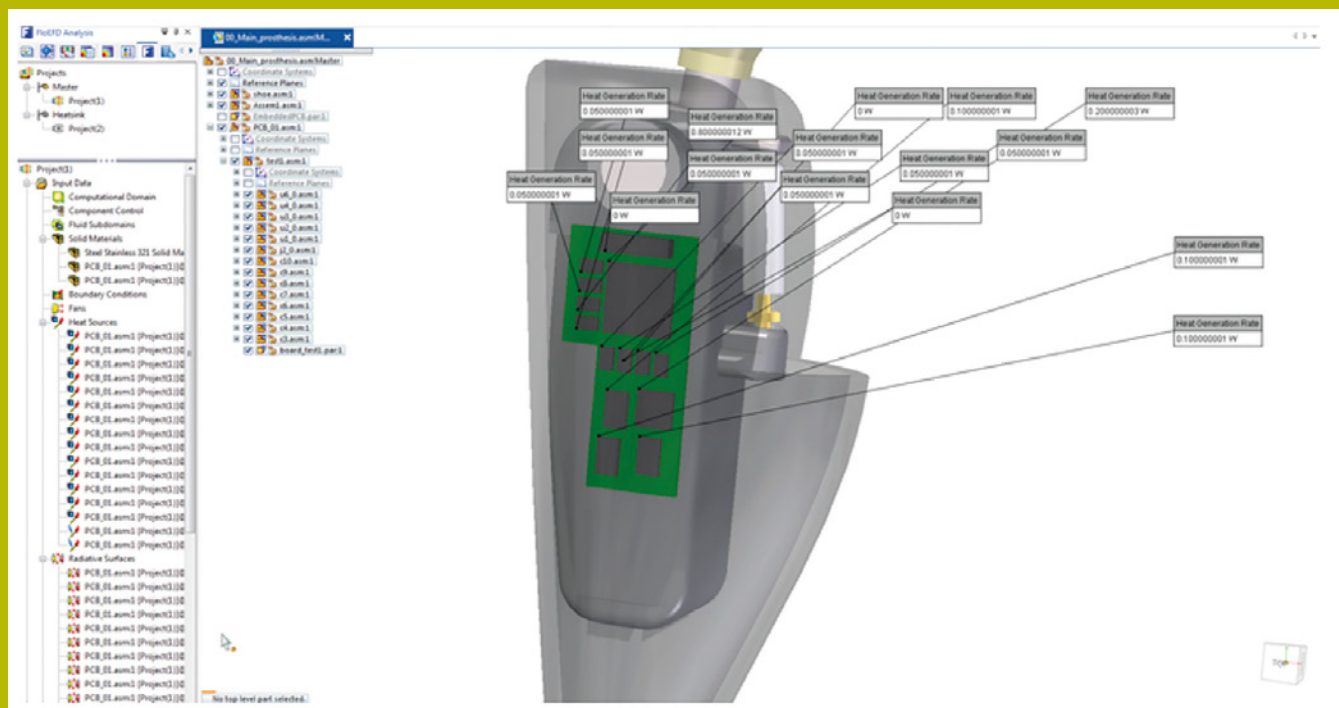
Figure 3: Boundary conditions of the PCB
