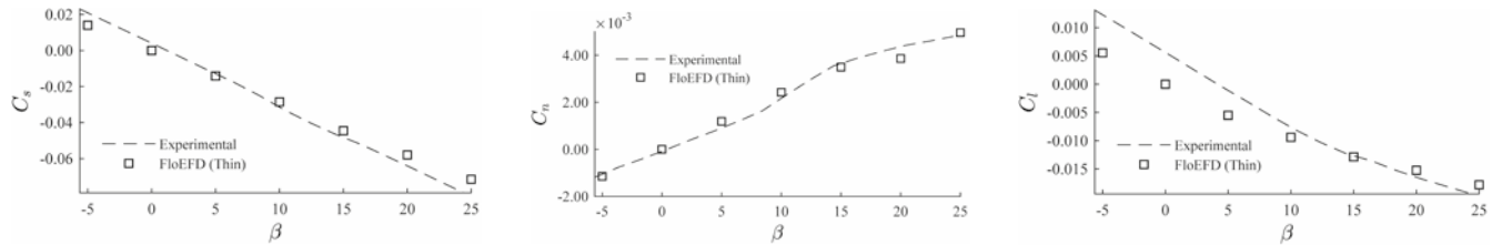
Figure 5: Comparison of Side Force, Yawing and Rolling Moment coefficients
