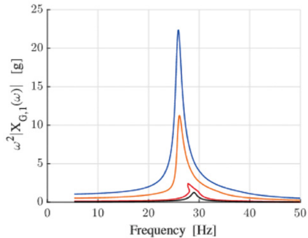
Figure 6: Amplitude of the harmonic forced response of Galileo in terms of acceleration using Simcenter Samcef Repdyn solver for several levels of base acceleration (black: 0.05 g, red: 0.1 g, orange: 0.5 g, blue: 1 g)
