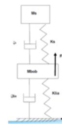
Figure 1: Test rig and numerical model for fixed / free beam
