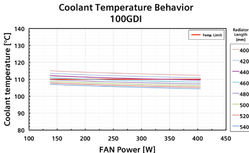
Figure 6: Coolant temperature, drive scenario F
