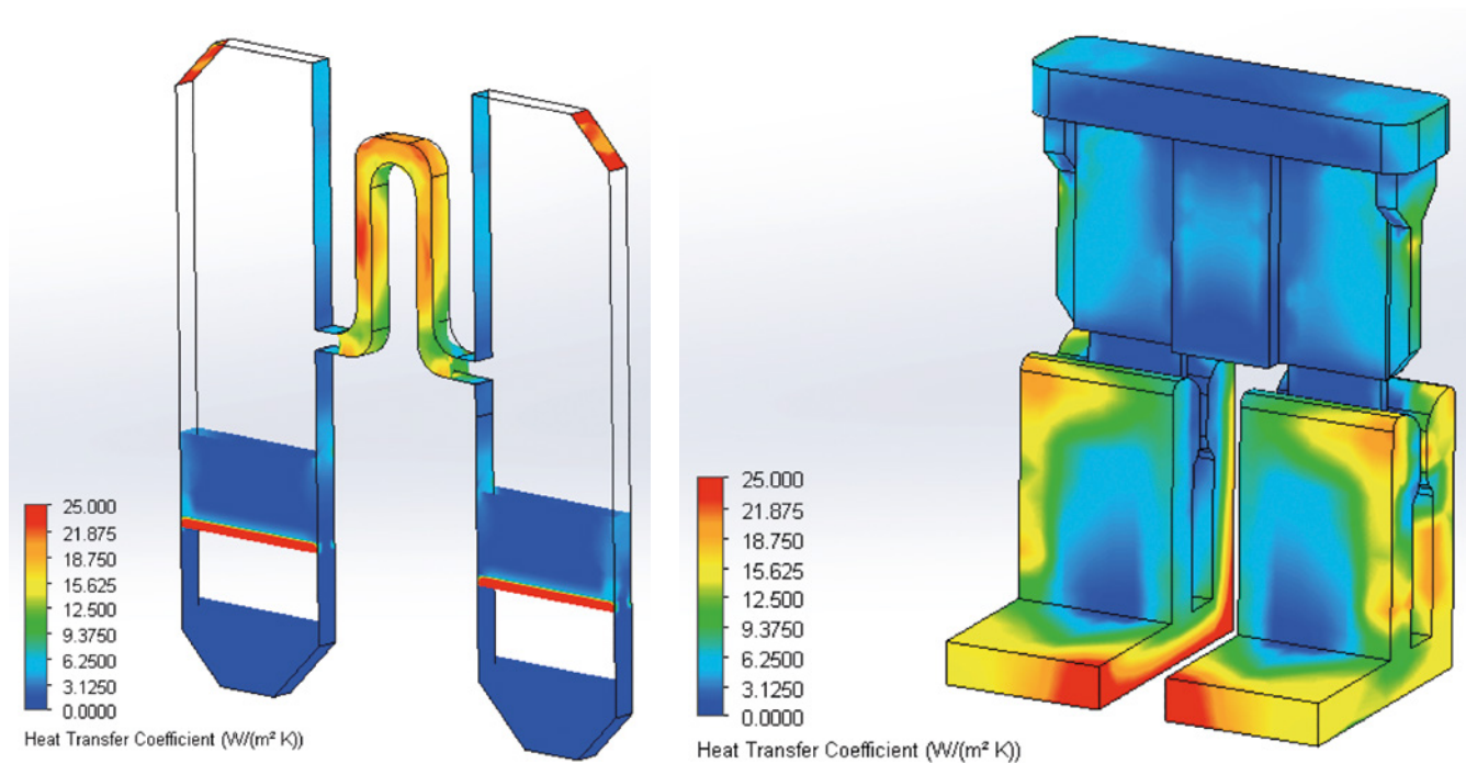
Figure 4: Local surface heat transfer coefficients on blade-type automotive 10A fuse
