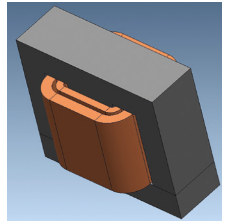
Figure 2. Full 3D FEM model of the single-phase shell type bench transformer
