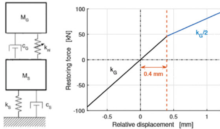
Figure 5: Modification of the structural model to account for the loss of stiffness.
