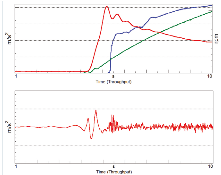
Figure 3: Vehicle acceleration maneuver in hybrid mode: combustion engine restarts to charge the battery after initial pure electric propulsion, generating body vibrations.
