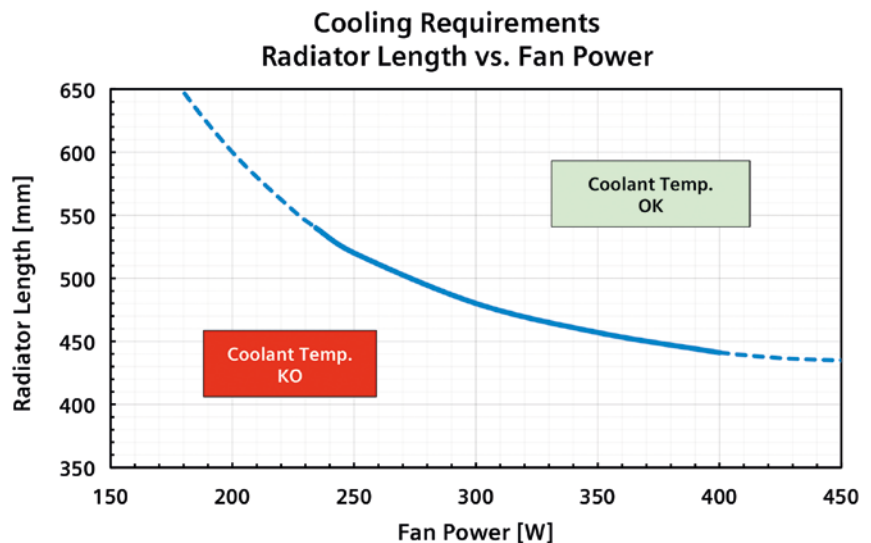
Figure 8: Cooling requirements according to all driving conditions
