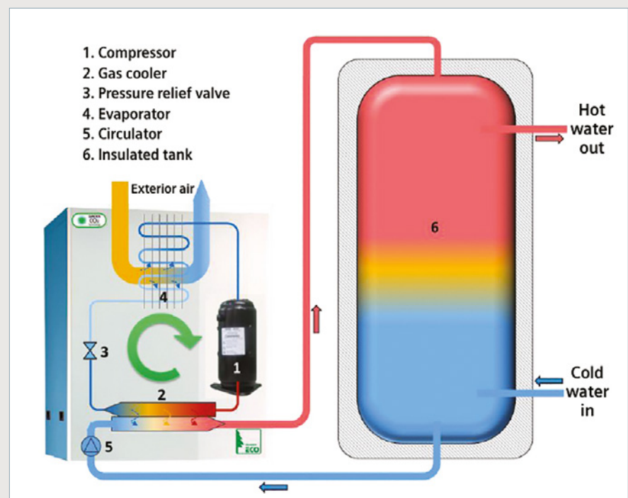
Figure 1: Schematic of a CO 2 -based air/water heat pump.
