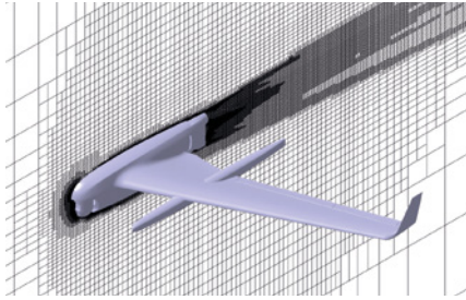
Figure 1: Cartesian Mesh used in the numerical model for the sUAS.
