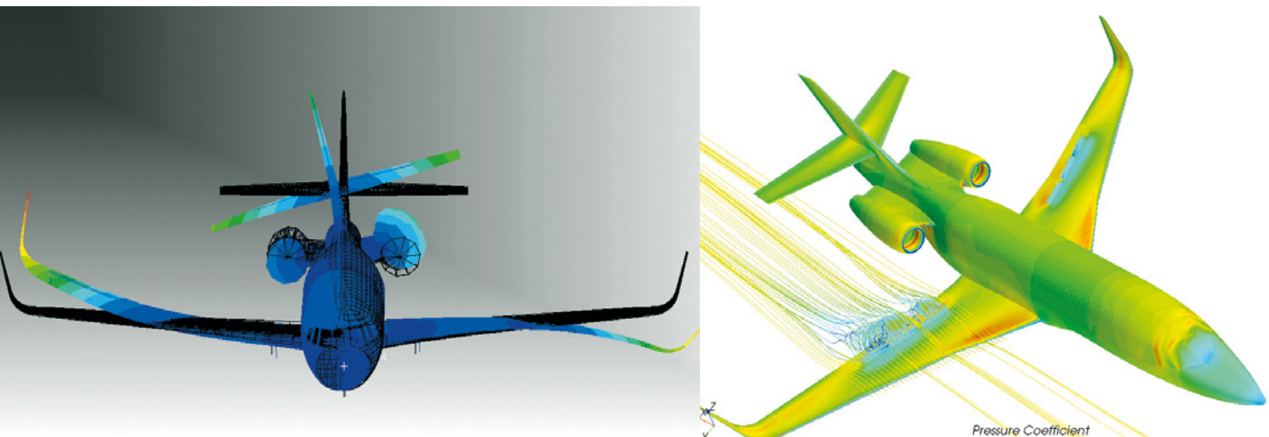
Figure 1: For airplanes where structural flexibility is important, a coupled aerodynamic and structural certification-by-analysis approach is needed.
