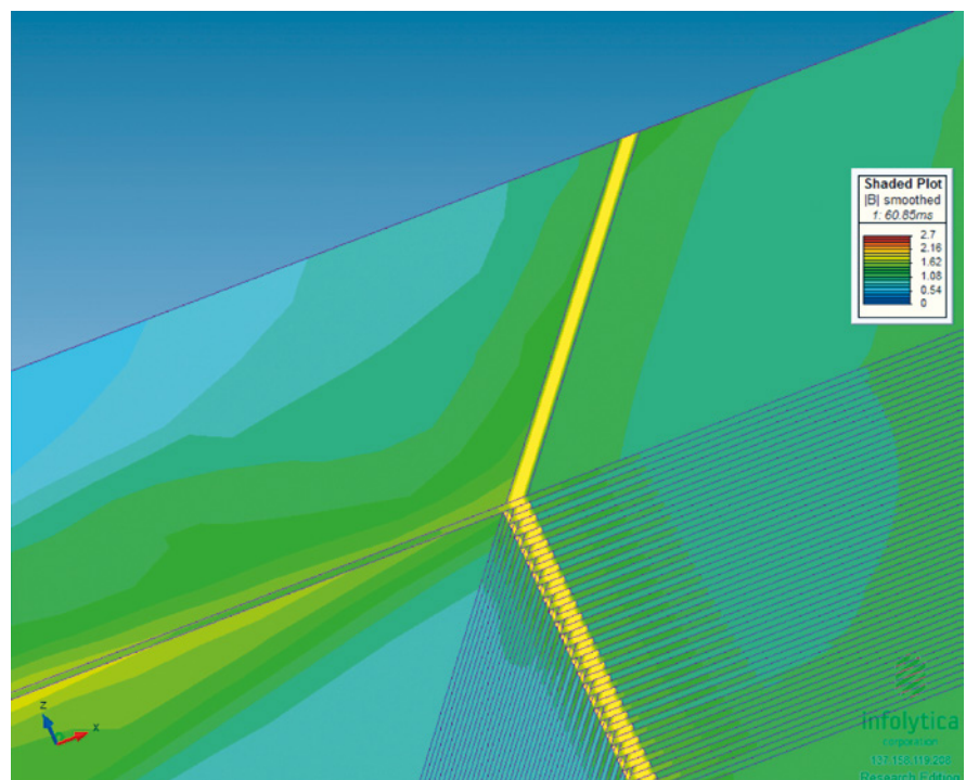
Figure 7. Core stacking lamination detail close to the surface of a mostly solid core.
