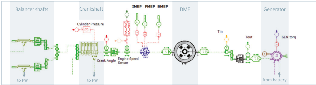
Figure 2: Hybrid driveline torsional model including combustion engine and generator to study ICE restart vibrations.
