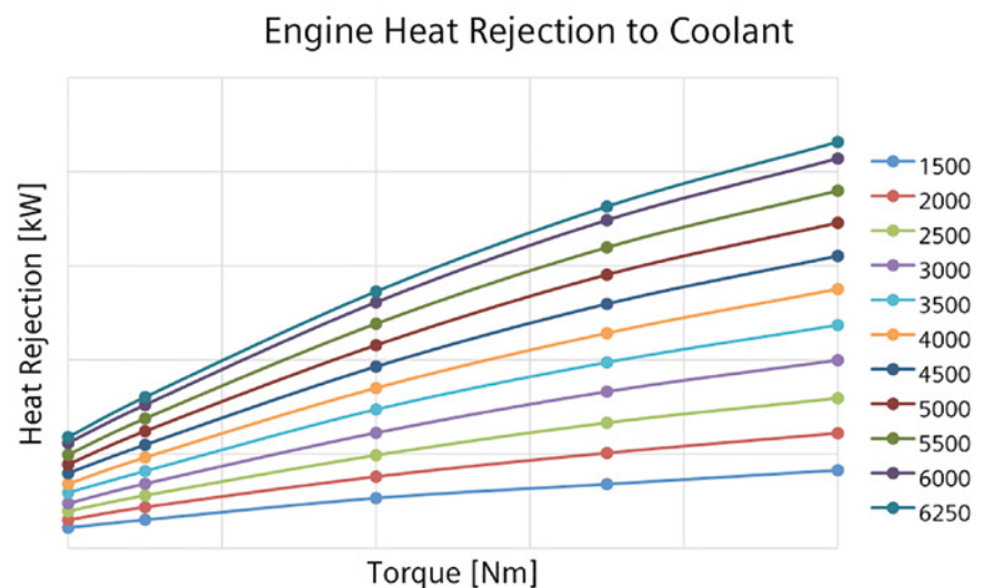
Figure 2: Heat rejection map
