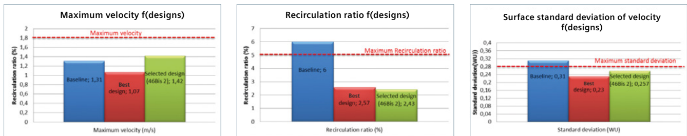
Figure 7: Performance comparison of baseline and Design Manager improved designs, in addition to selected “final” design.
