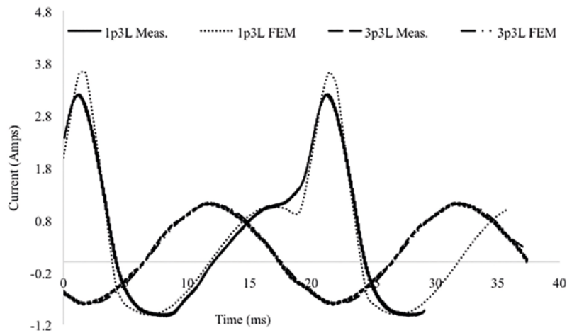
Figure 4. Primary current waveforms for 1p3L and 3p3L test transformers with 550 mA DC and 160 mA DC per phase respectively
