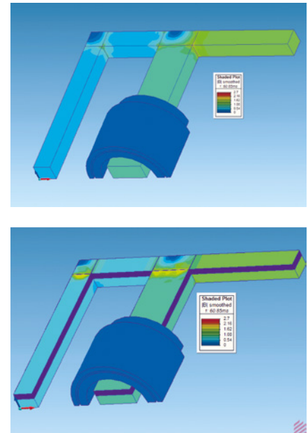
Figure 6. Flux distribution at normal AC excitation for calibrating the FEM model of no load current with measurements. Left: core modeled as solid with air gaps at the joints. Right: core modeled with explicit 0.3 TKES H111-30 grain oriented electrical core steel laminations stacked close to the core surface.
