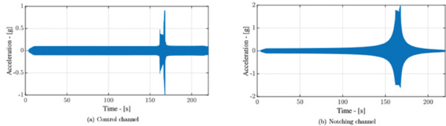
Figure 8: Control and notching channel in time domain
