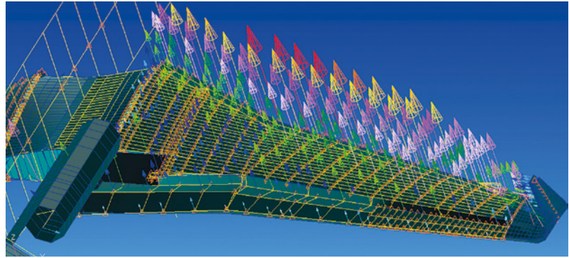
Figure 3: Certification by analysis at TLG starting with the aerodynamic database generation with Simcenter STAR-CCM+, mapping results to NASTRAN with DLM and the final aeroelastic model in NASTRAN
