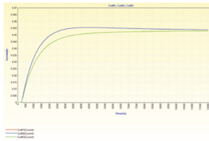
Figure 5. DC time response of the 3p5L model transformer with 160 mA in the neutral
